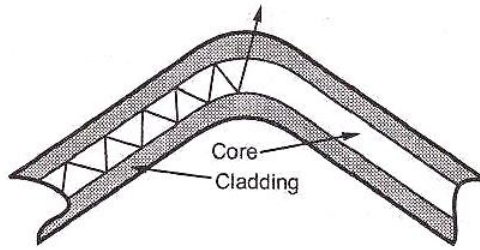
Figure: Macrobending Loss
