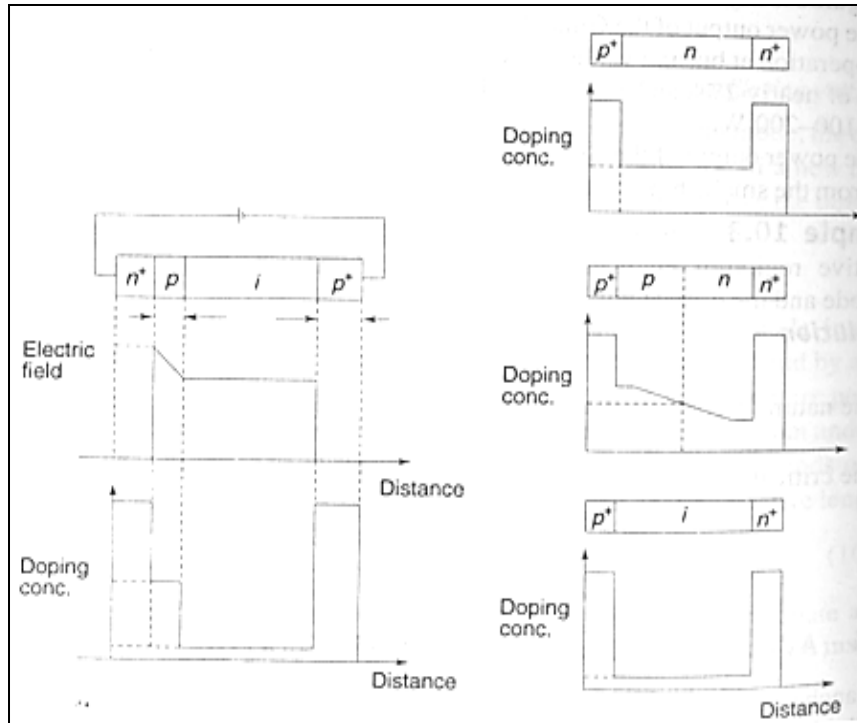
Fig; Various structures of IMPATT diode
