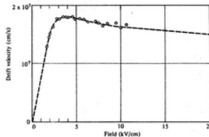
Fig; Drift Velocity of n-type Ga-As Vs Electric Field
