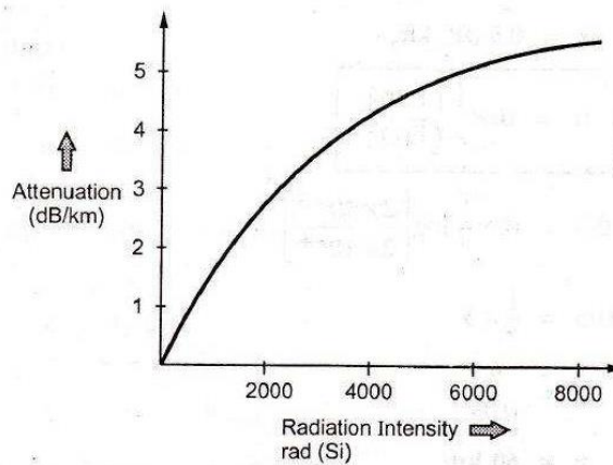
Fig: Ionizing Radiation intensity Vs Fiber Attenuation
