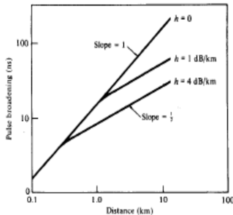
Fig: Mode coupling effects on pulse distortion in long fibers for various coupling losses
