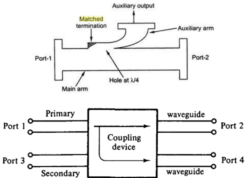
Fig Directional coupler.
