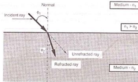
Fig: Refractive Model for Snell's law
