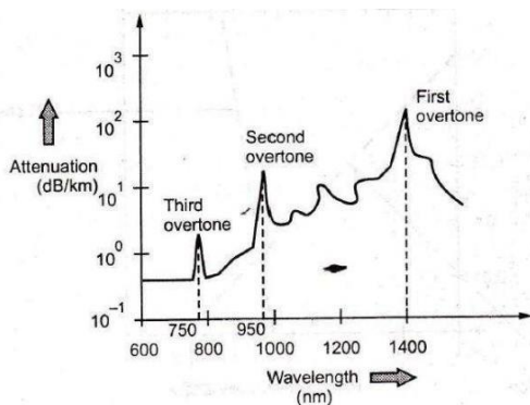
Fig: Absorption Spectra for OH group
