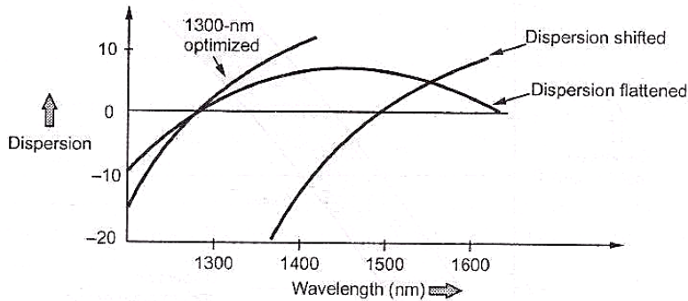
Fig: Total Resultant Dispersion Dispersion Calculations
