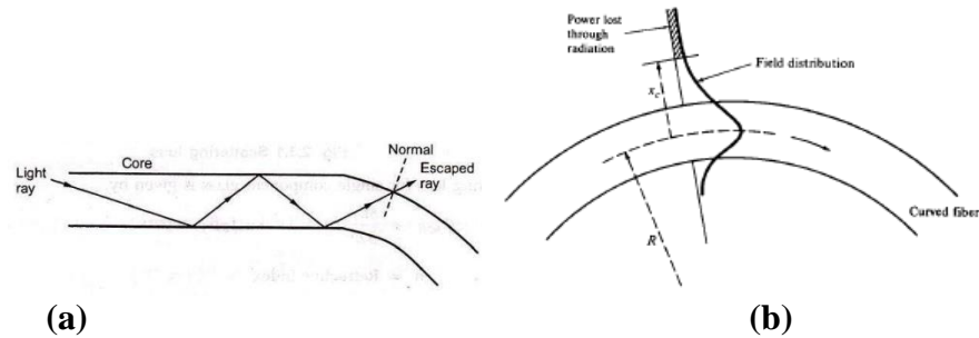
Figure: Bending Loss
