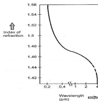
Fig: Index of refraction as a function of wavelength
