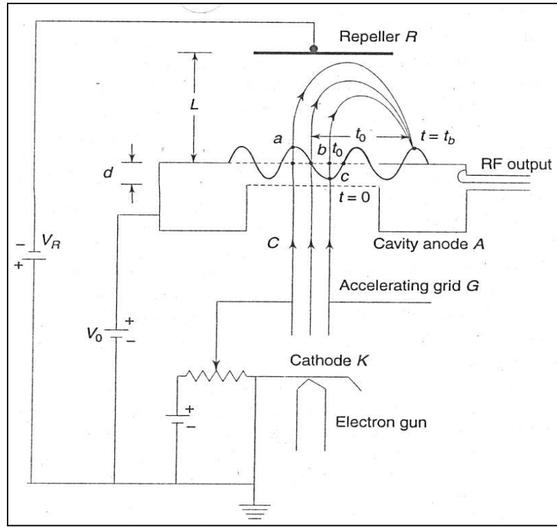
Fig.: Schematic diagram of Reflex klystron oscillator
