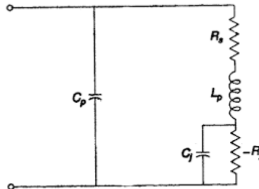
Fig: electrical equivalent circuit of a Gunn diode
