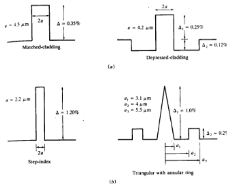
Fig: (a) 1300 nm – Optimized (b) dispersion-shifted
