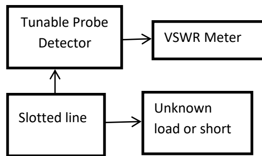
Fig: Determination of load impedance using slotted line
