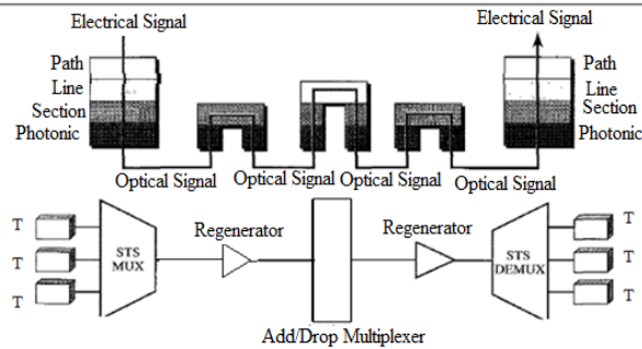
Figure 1.22 Device-Layer Relationship in SONET
