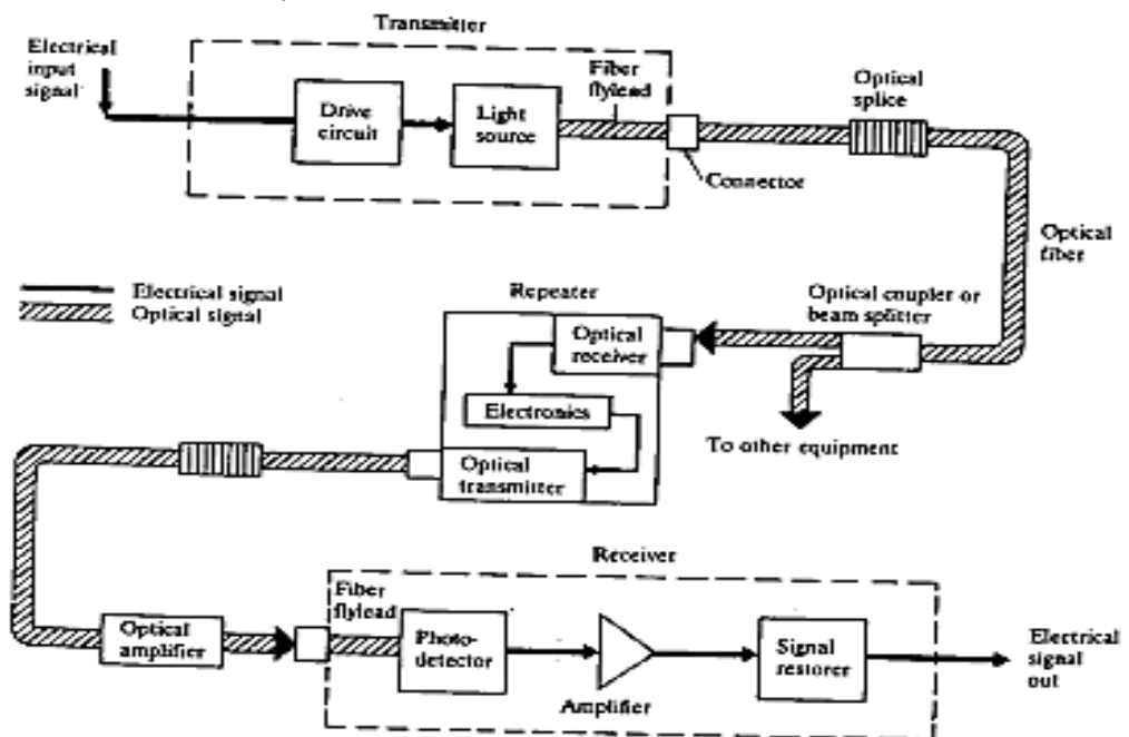
Fig: Major Elements of a Optical Fiber Transmission Link
