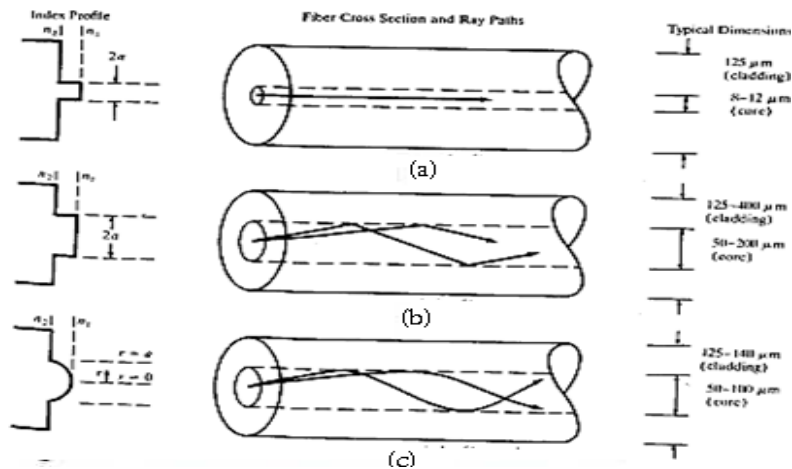
Fig (a) Single mode step index Fiber (b) Multimode Step-index Fiber (c) Multimode graded-index Fiber
