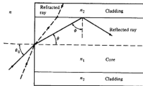
Fig: Meridional Ray optic representation of the propagation mechanism
