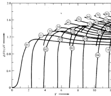
Fig: Group Delay of waveguide dispersion as function of V number of step-index fiber Refractive Index Profile
