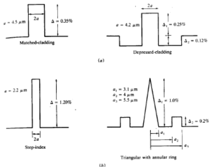
Fig: (a) 1300 nm – Optimized (b) dispersion-shifted
