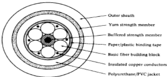
Fig: Six Fiber cable
