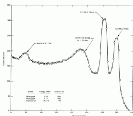
Compton edge of ^{60}\text{Co} on gamma spectrometer Na(Tl).
