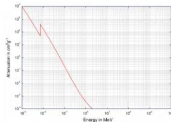
Cross section of photoelectric effect.
