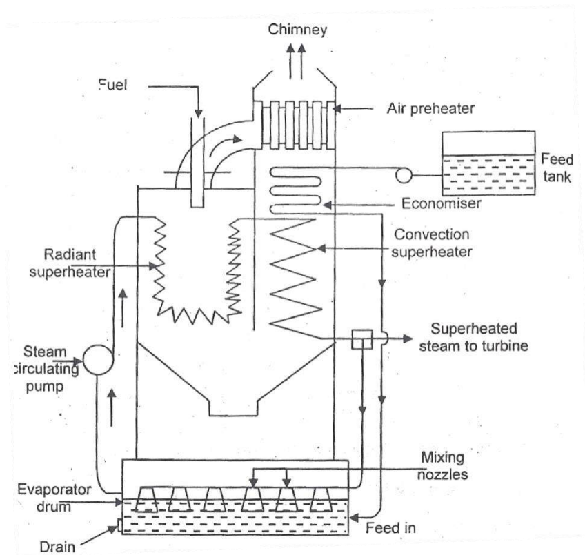
Loeffler boiler
