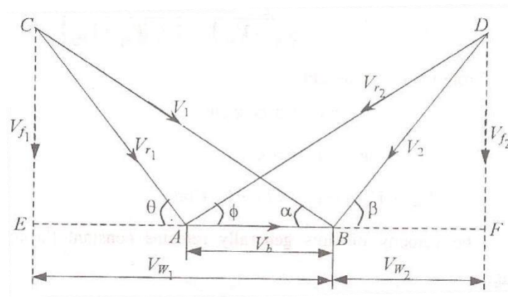
Velocity diagram for reaction turbine
