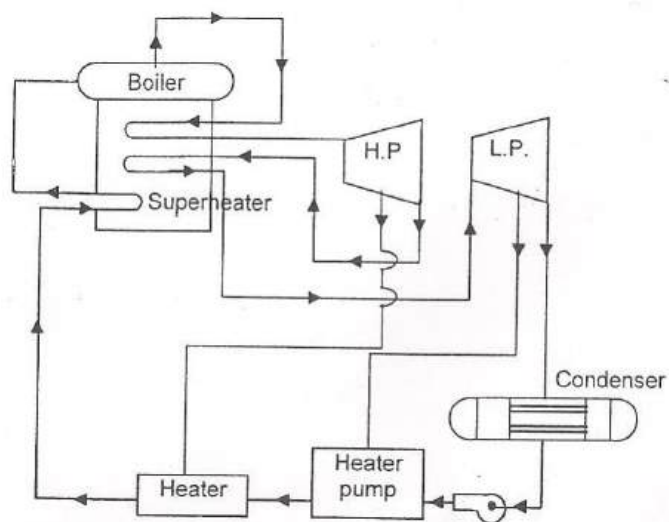
Reheat-Regeneration cycle
