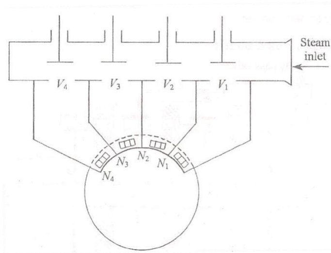
Nozzle control governing
