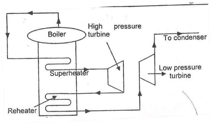
Flue gas reheating
