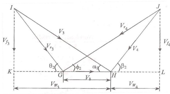
Velocity diagram for the second row of moving
