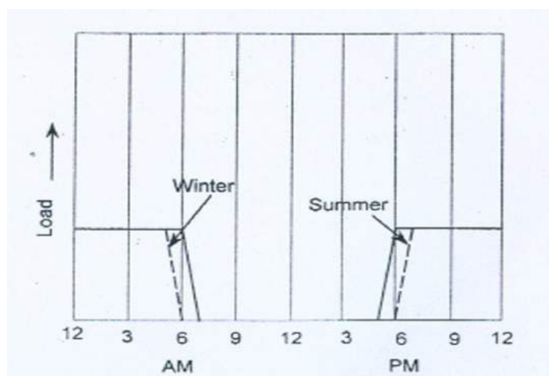
Street lightning load curve
