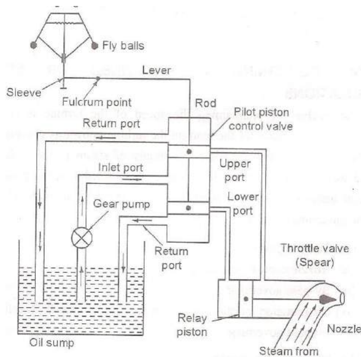
Throttle governing
