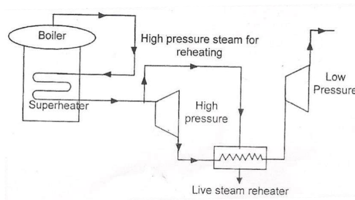
Live steam reheating
