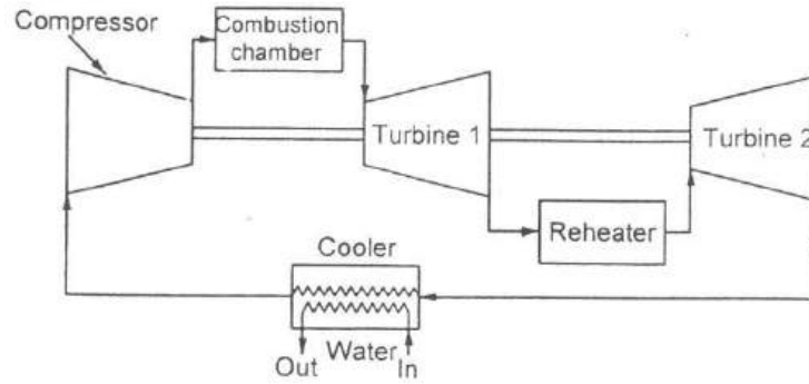
Fig. 4.25(a) Brayton cycle with reheater
