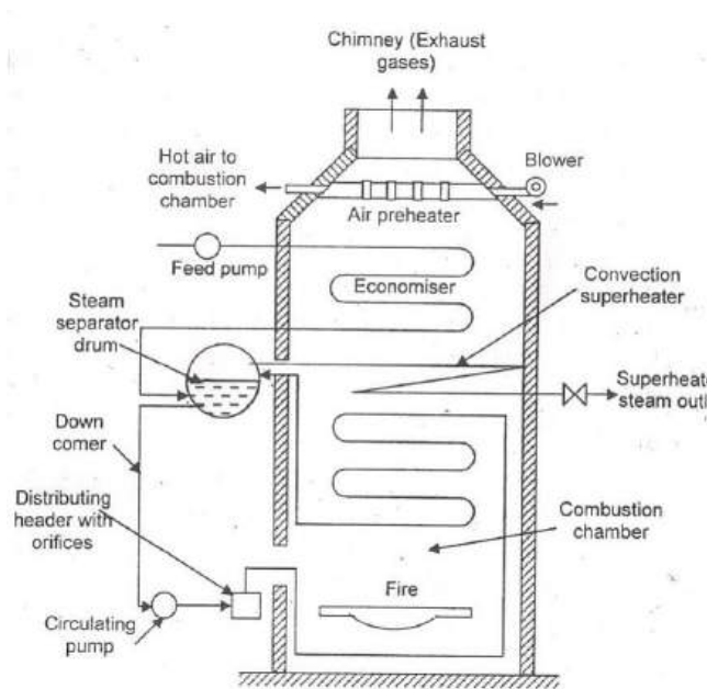
La-Mont Boiler
