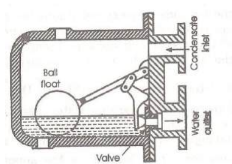
Ball float steam trap
