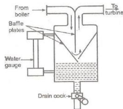
Steam separator
