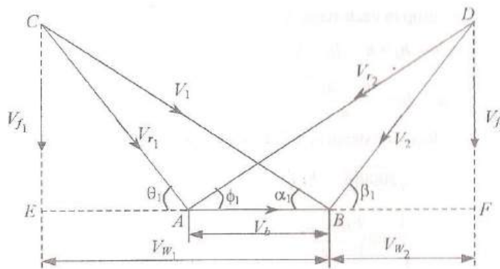
Velocity diagram for the first row of moving blades
