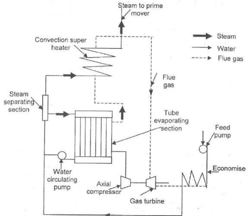
Velox boiler
